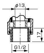
DETAIL "C"
